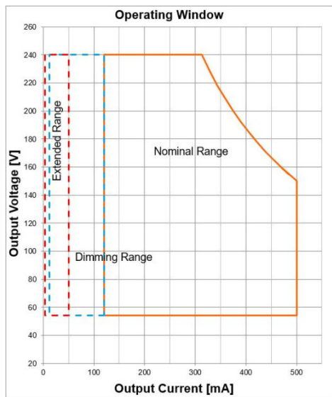
Operating window ETI DALI 75220-240500 D LT2 L
